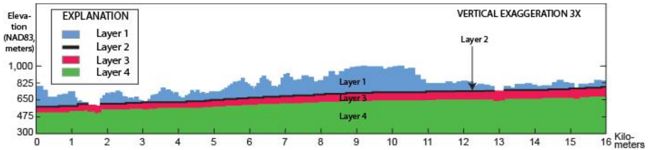
Figure 6. Cross section showing layers of the numerical groundwater-flow model developed for the Elkhorn Area, WV.
