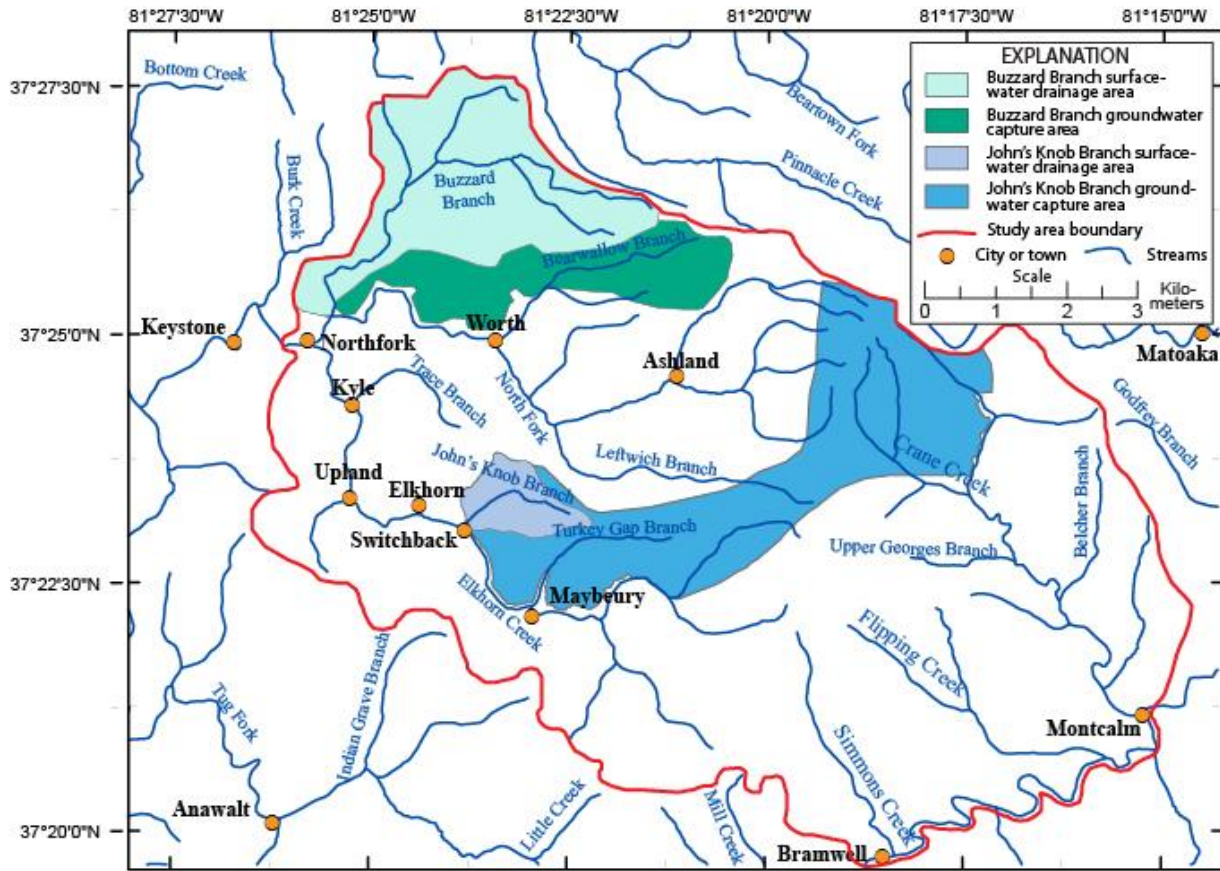
Figure 5. Surface-water drainage areas and estimated groundwater capture areas required to produce measured flows for Johns Knob Branch and Buzzard Branch, in the Elkhorn area, WV. [Bedrock and coal seams dip from east to west].
